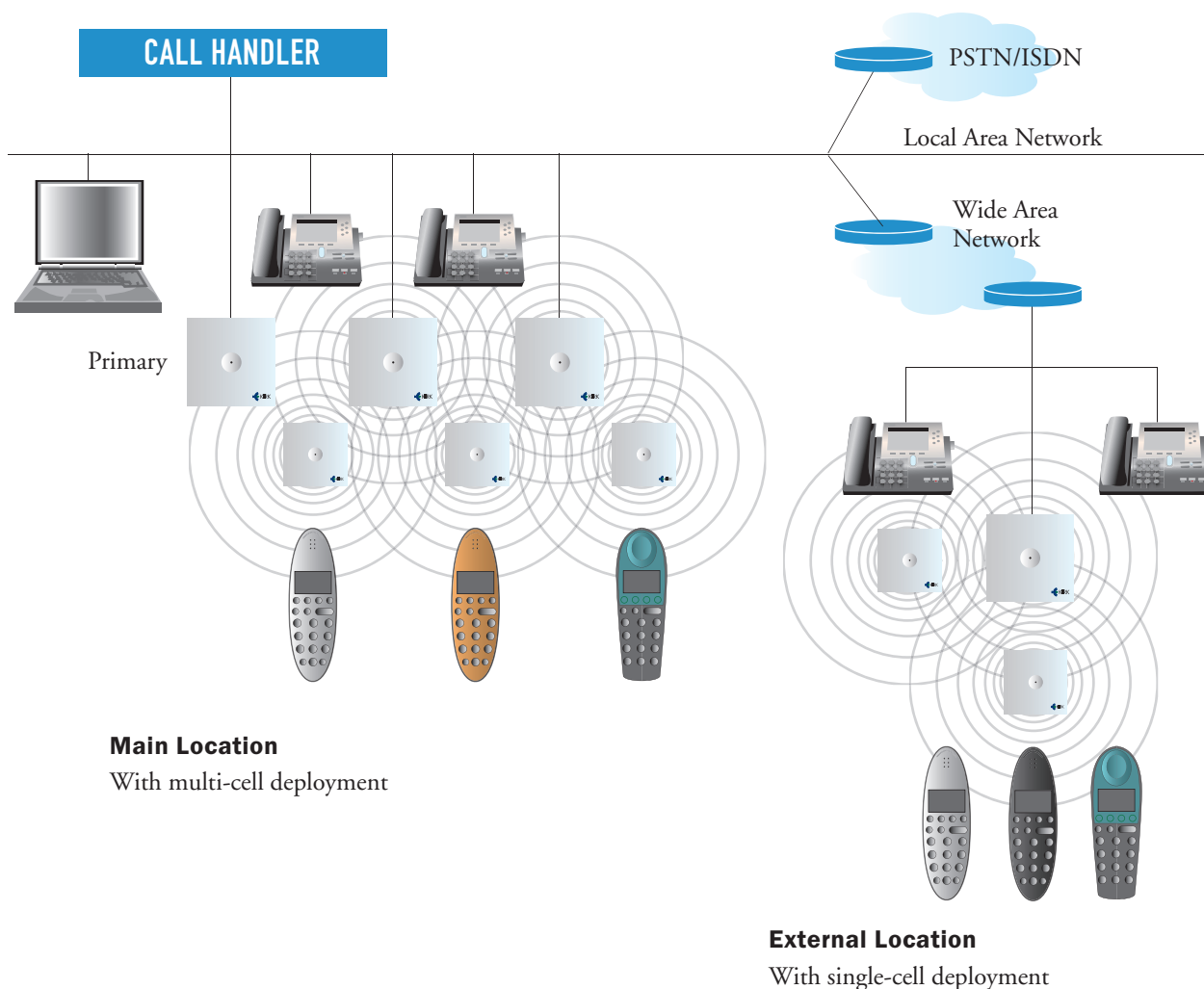
Figure 1 Overview of the Whole Solution
